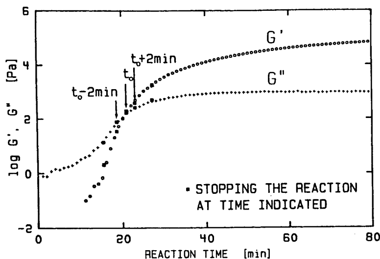
Figure 1. Evolution of the complex shear modulus, G' and G'' during cross-linking of PDMS at 34^{\circ}\text{C} , \omega = 0.5\text{rad/s}
