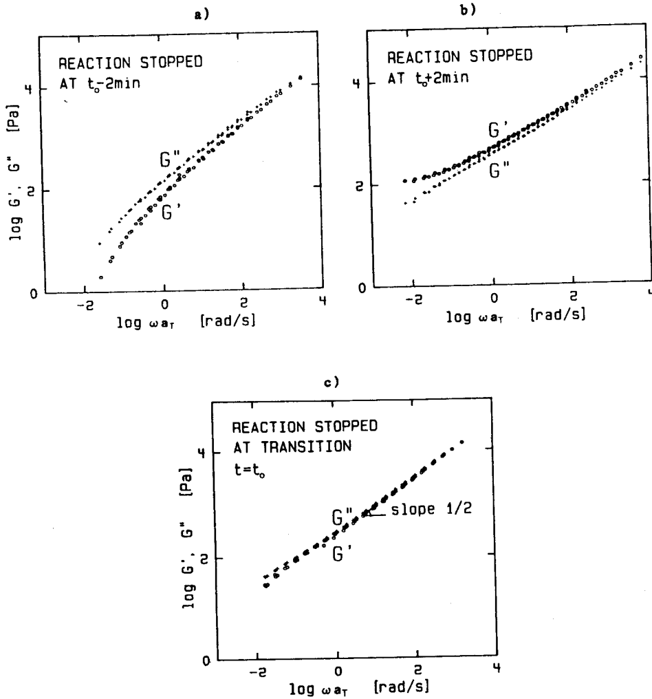
Figure 2. Evolution of the storage G' and loss G'' moduli. Master curves reduced at 34^\circ\text{C} a) 2 minutes before the transition state b) 2 minutes after the transition state c) the transition state (very slightly before)
