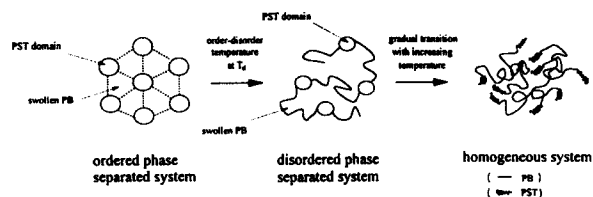
Figure 6 Schematic evolution of the structure of a non-annealed sample on heating
