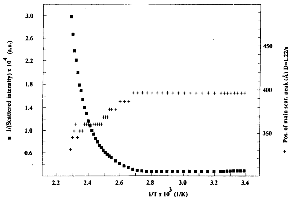
Figure 2 Reciprocal intensity plot for SEBS-20%, deduced from Figure 1
